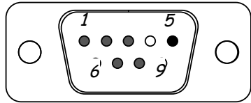
Rear View
