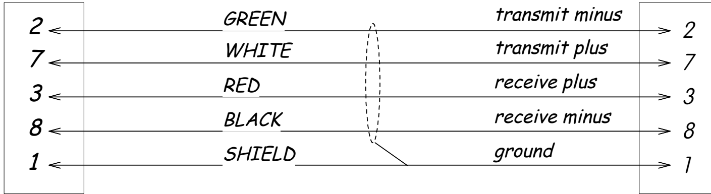
Solder View
