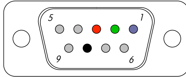
Solder View
